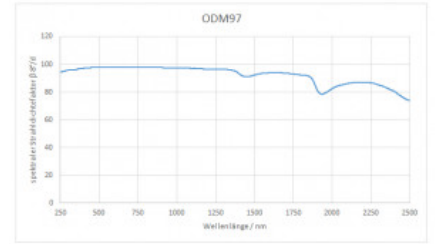
Wavelength / nm - Typical Spectral Reflectance
